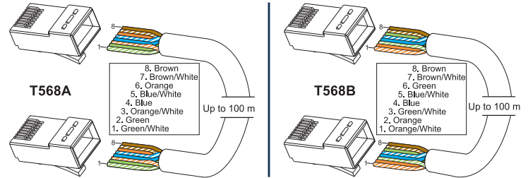
FIG. 5 RJ-45 CONNECTOR PINOUTS
