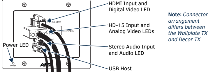
FIG. 8 ATTACH SIGNAL AND CONTROL CABLE (WALLPLATE TX SHOWN)
