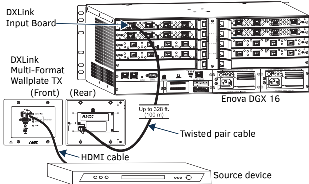
FIG. 2 WALLPLATE TX (FRONT & REAR) USED W/DXLINK INPUT BOARD IN ENOVA DGX 16
