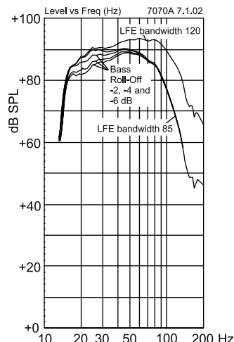
Figure 10. The free field frequency response of 7070A and 7071A subwoofers at different Bass Roll-Off settings.
