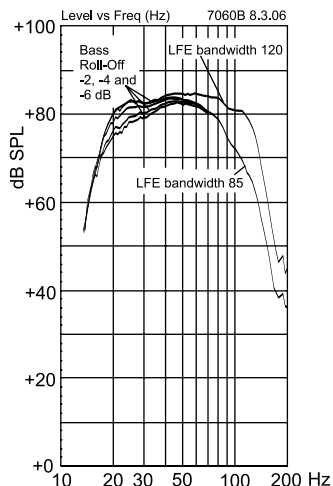
Figure 9. The free field frequency response of the 7060B subwoofer at different Bass Roll-Off settings
