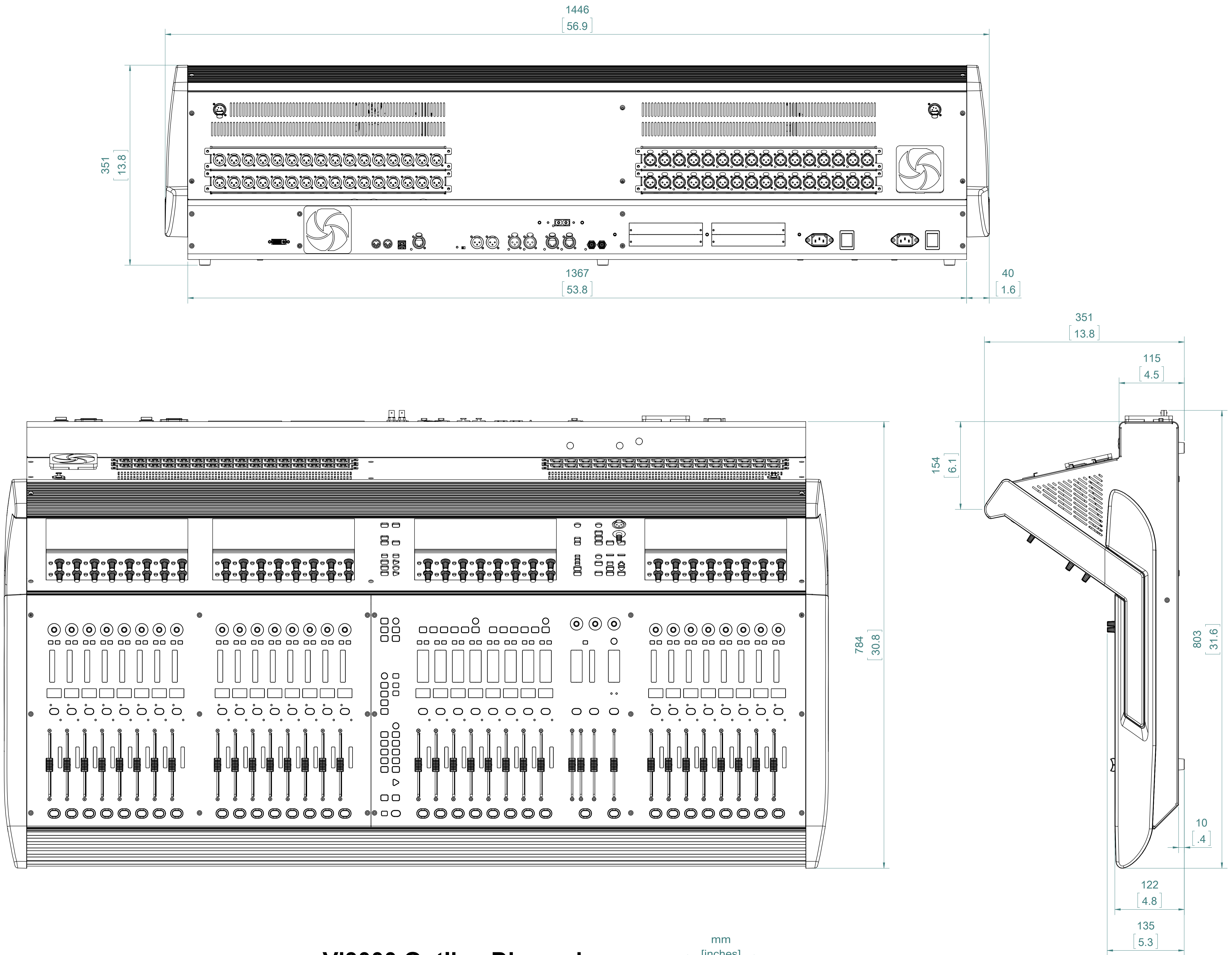
Vi3000 Outline Dimensions
