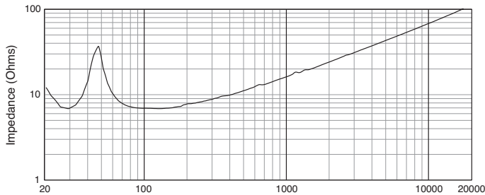
VT4881A Impedance
