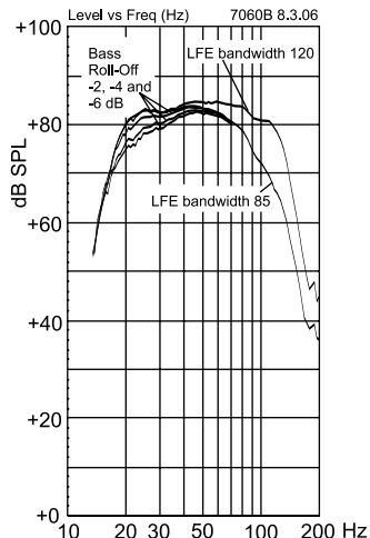
Figure 9. The free field frequency response of the 7060B subwoofer at different Bass Roll-Off settings
